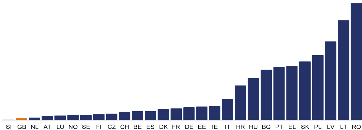
Figure 4.8 Trespasser safety risk (FWSI for trespassers per train-km) by European country, 2020 to 2024 average
