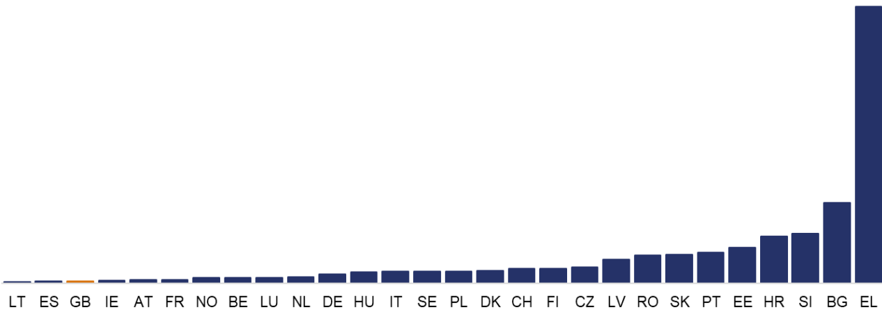
Figure 4.5 Employee safety risk (FWSI for employees per train-km) by European country, 2020 to 2024 average
